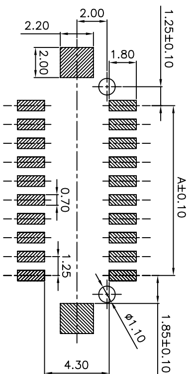
PCB LAYOUT
